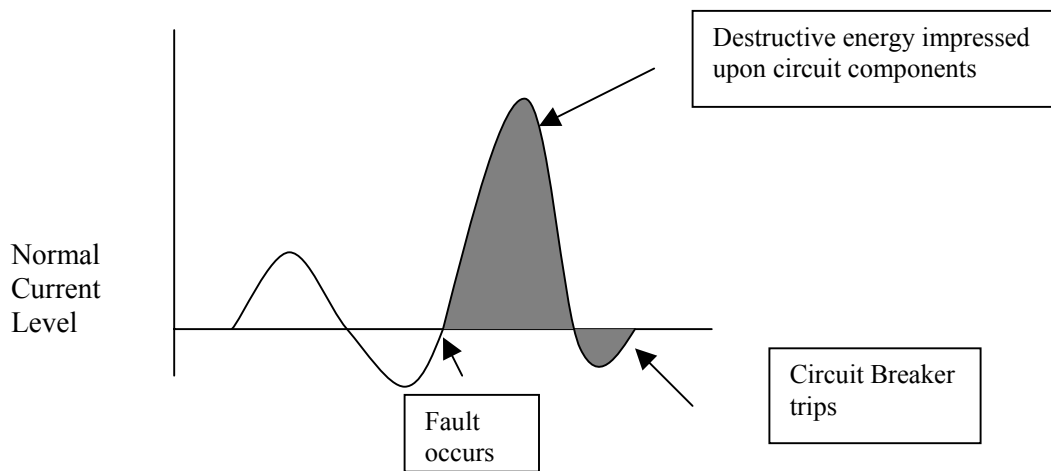
Figure 1. Current build up allowed by a non-current-limiting device releasing a large amount of destructive short circuit heat energy before opening.
