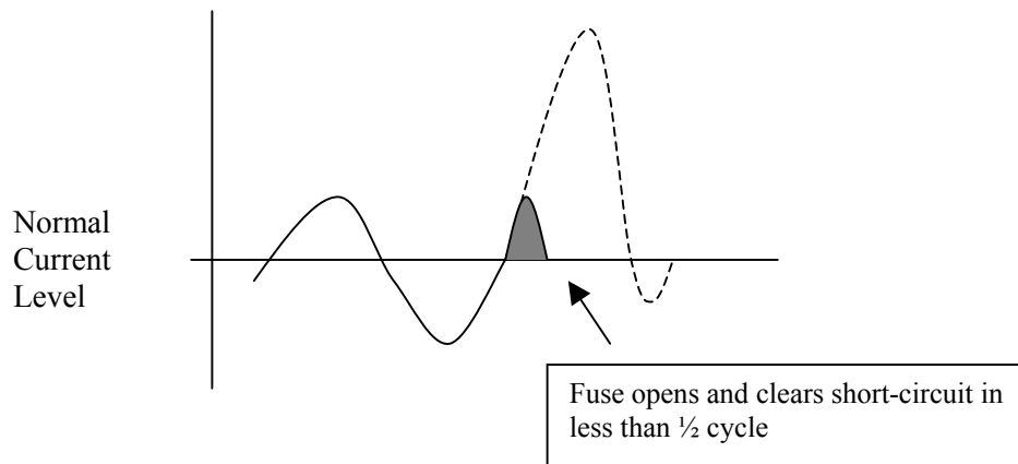
Figure 2. High-speed response of the current limiting fuse does not allow current build up to peak value
